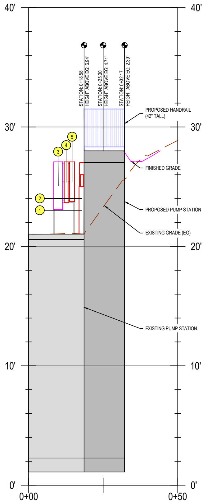
PUMP STATION 20 SURFACE IMPROVEMENTS PROFILE
